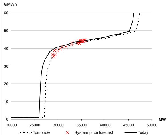
Supply curve and system price
